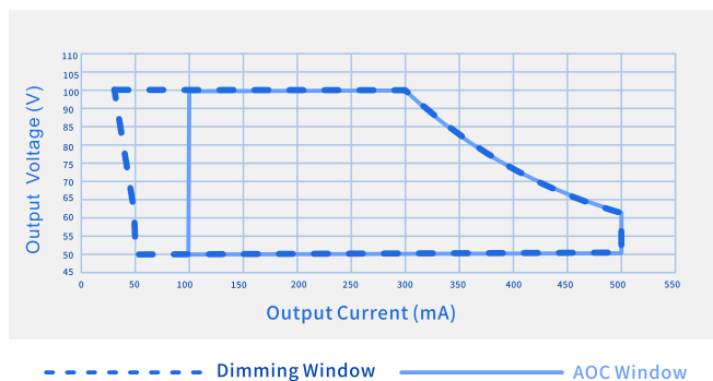
Output Voltage Vs. Output Current(Dim/AOC Window)
