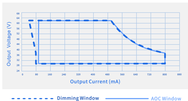
Output Voltage Vs. Output Current(Dim/AOC Window)
