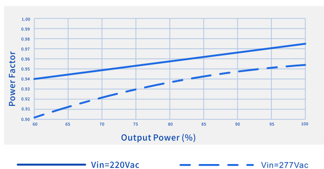
Power Factor Vs. Output Power
