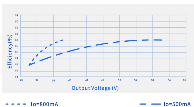
Efficiency Vs. Output Voltage (Vin=220Vac)
